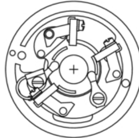
VIEW OF BRUSH ASSEMBLY INSTALLED ON END PLATE 2 X SCALE
